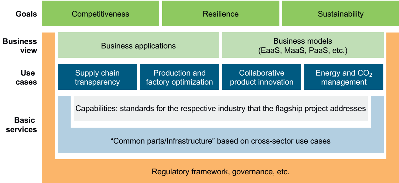
Figure 20: Proposed architecture for a Manufacturing-X flagship project
